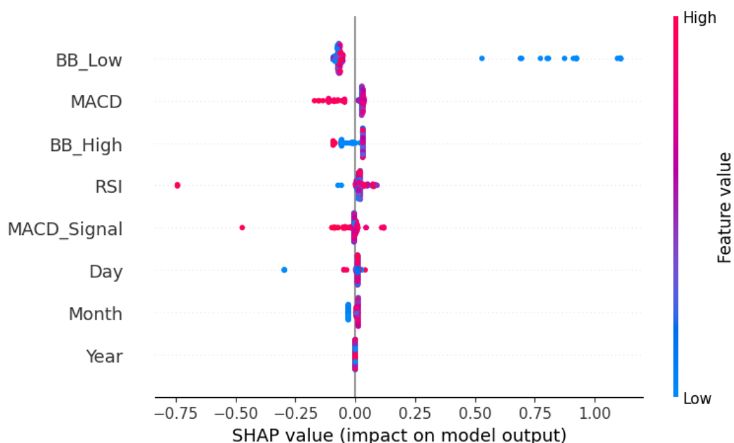
Diagram 24. Gradient Boosting SHAP Analysis Gradient Boosting SHAP Analysis
