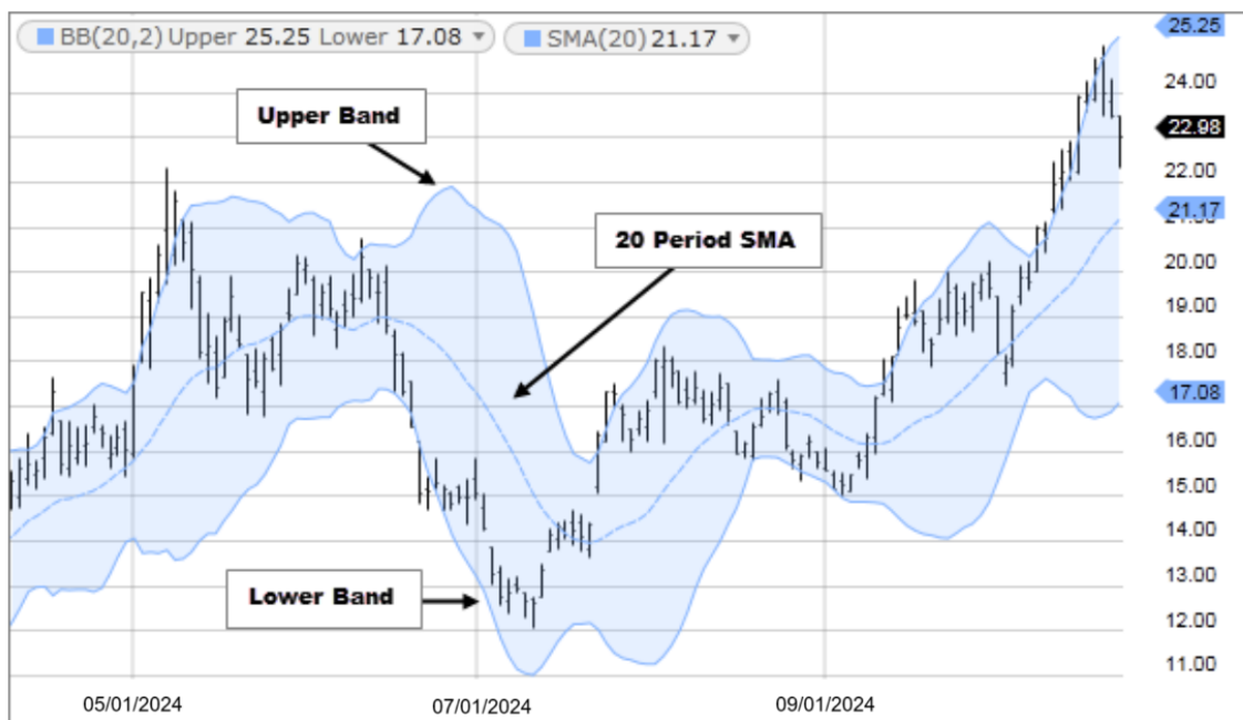
Diagram 3. Bollinger Bands indicator
