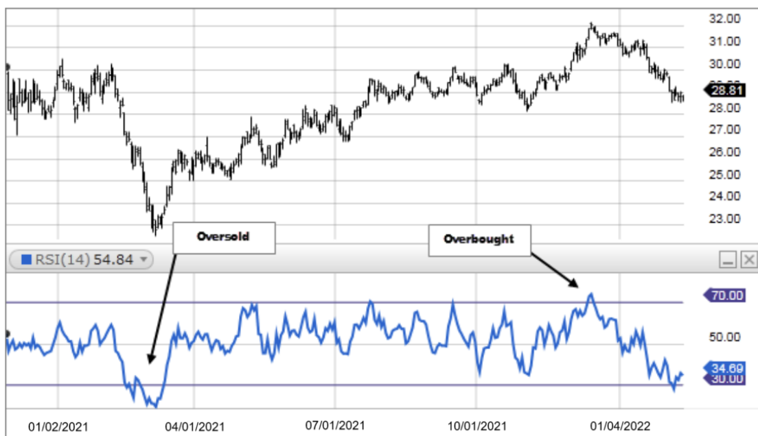
Diagram 1. Relative Strength Index (RSI)
