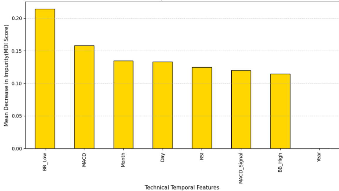
Diagram 20. XGBoost Feature Importance
