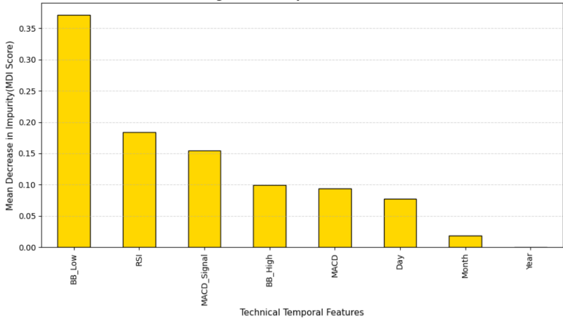
Diagram 21. Gradient Boosting Feature Importance Gradient Boosting Feature Importance - XAU/USD Framework
