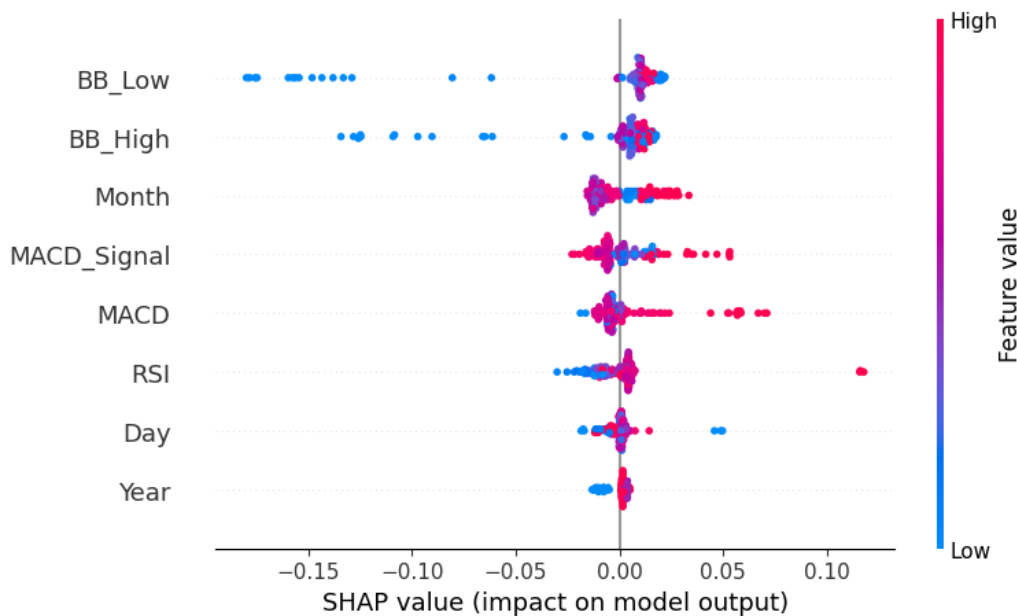
Diagram 22. Random Forest SHAP analysis Random Forest ShAP Analysis
