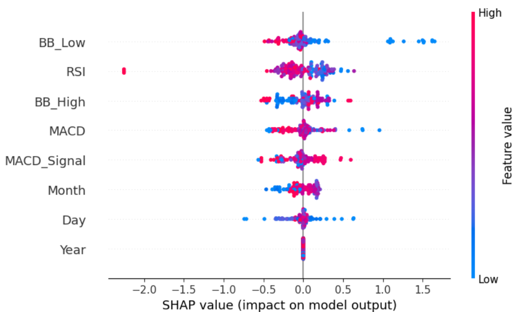
Diagram 23. XGBoost SHAP Analysis XGBoost SHAP Analysis
